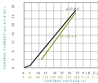
INPUT CURRENT VS CONTROL VOLTAGE(TYPICAL)
