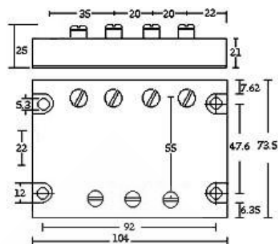
DIMENSIONAL DIAGRAM:
