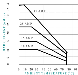
MAX ALLOWABLE CURRENT VS AMBIENT TEMPERATURE
